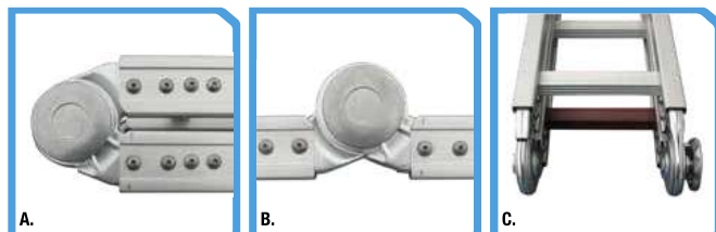
A. Closed articulated joint B. Open articulated joint C. Anodized red step
