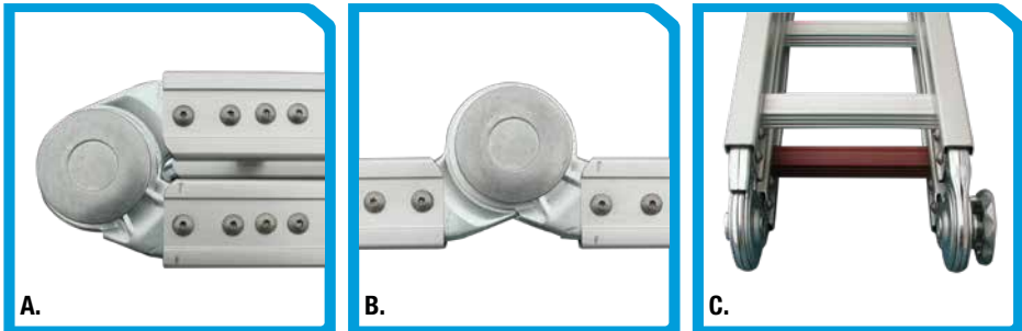
A. Closed articulated joint B. Open articulated joint C. Anodized red step
