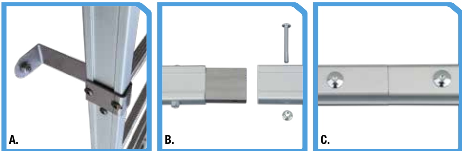
A. 150 mm bracket detail B. Graft C. Fixing after grafting
